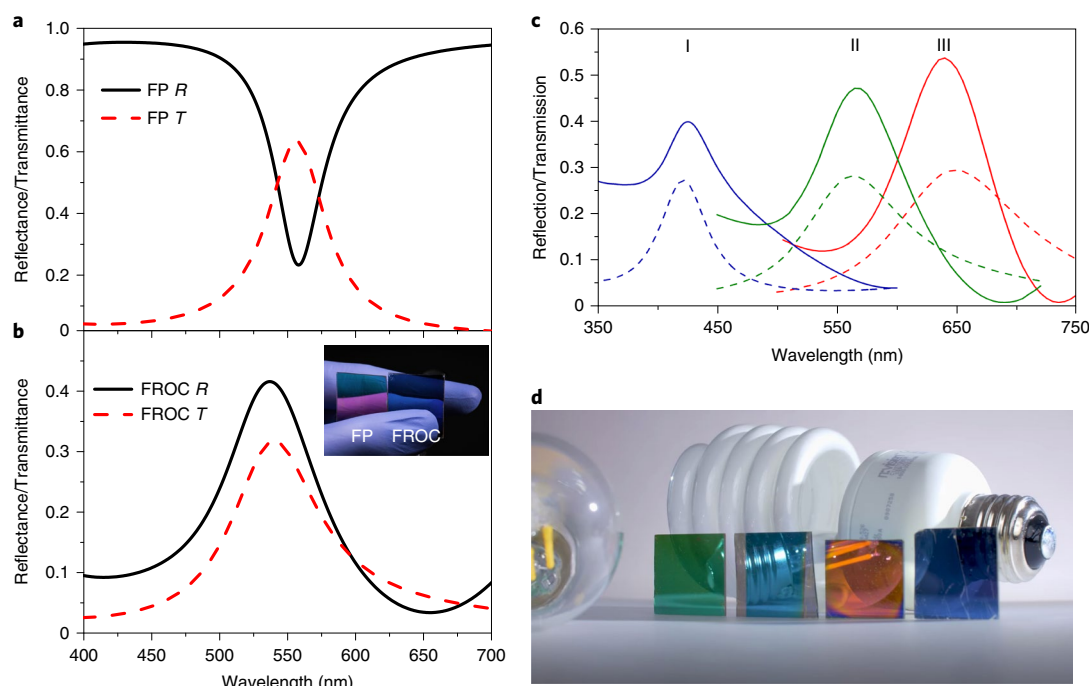
Fig. 3 | FROC as a beam splitter filter. a,b , Calculated reflectance and transmittance of a transmission filter based on an Fabry–Perot (FP) cavity consisting of a metal–dielectric–metal stack. (a) and (b) show the reflectance and transmittance for the MDM cavity, whereas for the FROC, both reflectance and transmittance peaks overlap. The inset in b shows a photograph of a conventional transmission filter and a BSF-FROC. The former reflects red while transmits green. The FROC, however, reflects and transmits the same blue colour. c , Measured transmittance (dashed lines) and reflection (solid lines) for three BSF-FROCs (Ge (15 nm)–Ag (25 nm)–PMMA (I, 100 nm; II, 120 nm; III, 170 nm)–Ag (25 nm)). d , Photograph of BSF-FROCs showing their potential for the structural colouring of transparent objects. The reflection of the incandescent bulb and transmission from the fluorescent light bulb have the same colour for each BSF-FROC filter.
