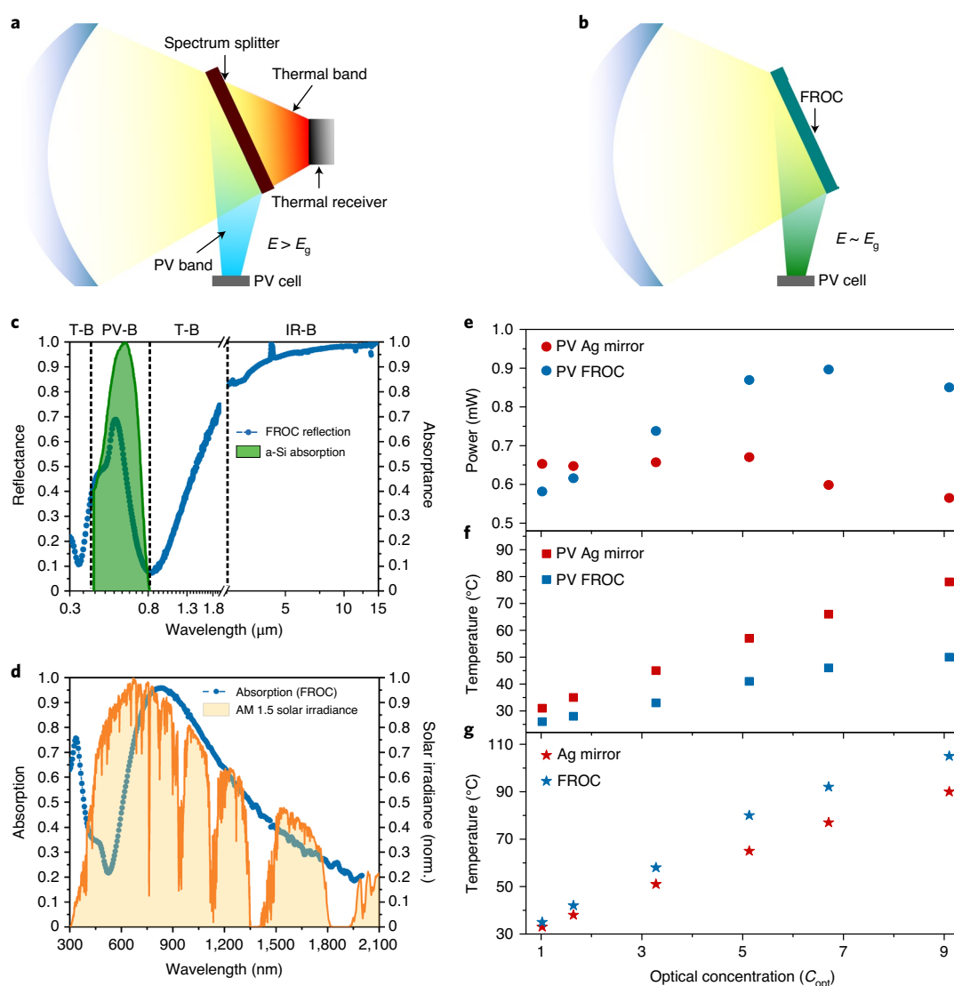
Fig. 4 | FROCs for hybrid thermal-electric solar energy conversion. a , Schematic of a conventional PV/solar-thermal energy conversion set-up in which concentrated solar light is incident on a spectrum splitting filter that reflects photons with energies greater than the PV bandgap energy E_g to a PV cell while transmitting the rest to a separate thermal receiver. b , A FROC, however, can reflect photons with energies close to E_g while directly absorbing photons E > E_g or E < E_g . c , Measured reflectance of a Ge(15 nm)-Ni(5 nm)-TiO 2 (85 nm)-Ag(120 nm) FROC that selectively reflects light within the wavelength range corresponding to the absorptance of an a-Si PV cell (green). T-B, PV-B and IR-B correspond to the thermal band, PV band and infrared band, respectively. d , The measured absorption of the same FROC shows overall high average absorption within the solar spectrum. The solar irradiance spectrum (AM 1.5) is shown for reference. e-g , For different optical concentrations C_{opt} we measured the power output from a PV cell receiving light reflected from an Ag mirror and the FROC ( e ), the temperature of the PV cell operating with an Ag mirror and the FROC ( f ) and the temperature of the Ag mirror and the FROC ( g ).
