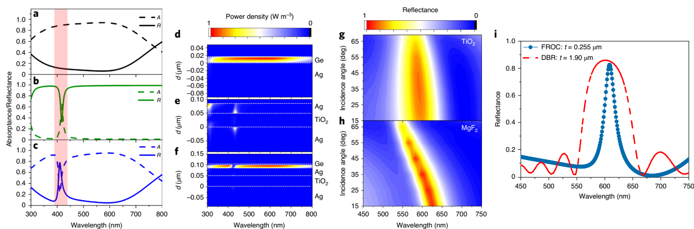
Fig. 2 | Demonstration and properties of Fano-resonant optical coatings. a–c , Calculated reflectance and absorptance A of a thin-film broadband light absorber ( a ), a narrowband light absorber ( b ) and a FROC ( c ). The highlighted region shows the spectral range where the narrowband light absorber resonance and Fano resonance take place. d–f , The calculated normalized power dissipation density in the three structures, highlighting the resonant destructive interference between the broadband and narrowband nanocavities. g,h , The measured angular reflection of a FROC with a high-index dielectric ( \text{TiO}_2 ; g ) and a FROC with a low-index dielectric ( \text{MgF}_2 ; h ). i , The calculated reflectance from a low-index contrast dielectric Bragg reflector with thickness t = 1.9 \mu\text{m} compared with the selective reflection of a FROC ( t = 0.255 \mu\text{m} ).
